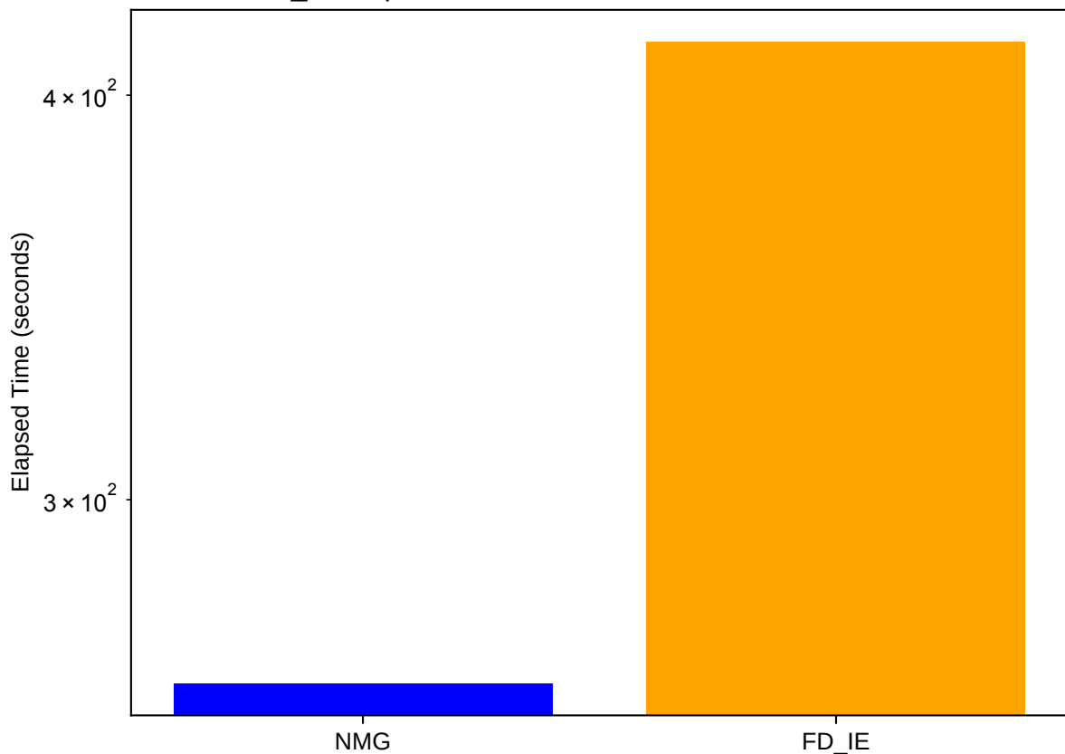
NMG vs FD_IE Elapsed Time for Neumann BC, 128x128 Grid, MATLAB
