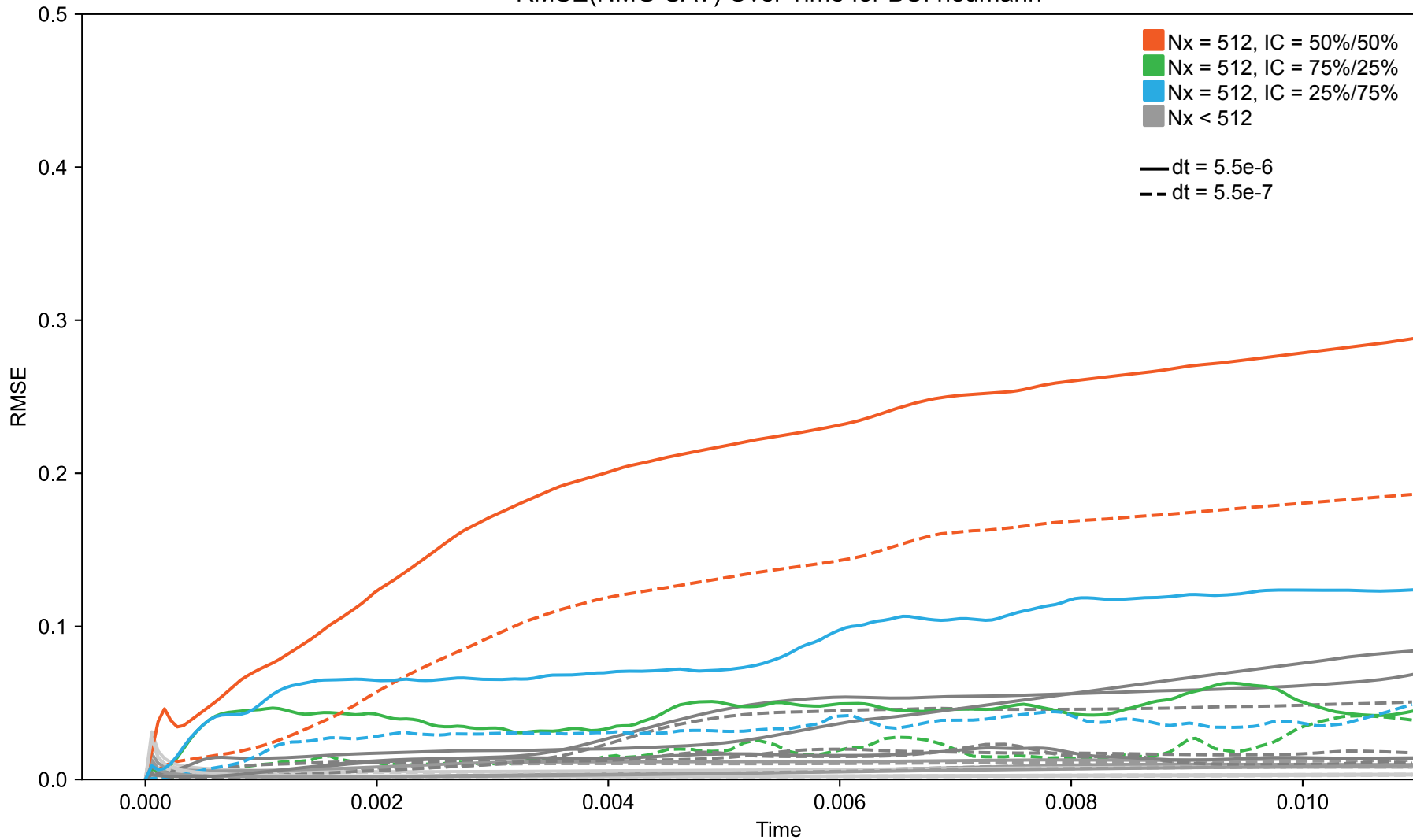
RMSE(NMG-SAV) Over Time for BC: neumann
