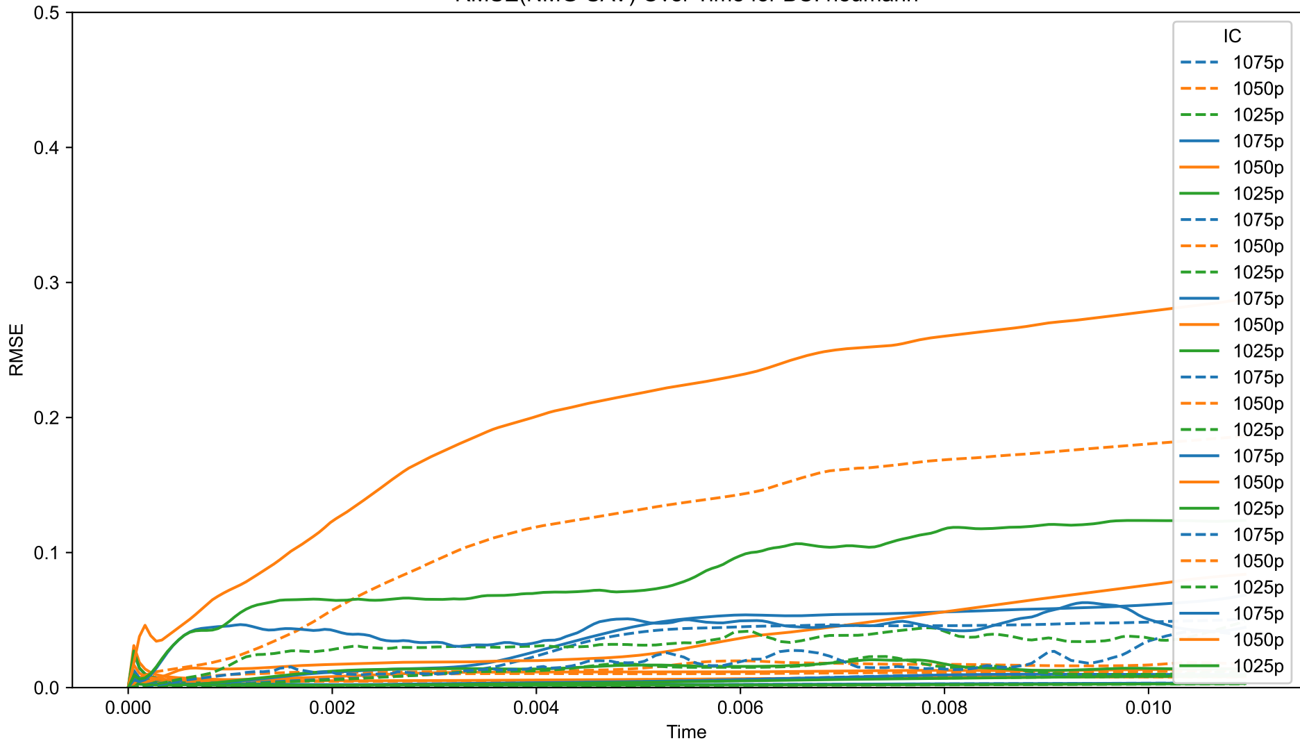
RMSE(NMG-SAV) Over Time for BC: neumann
