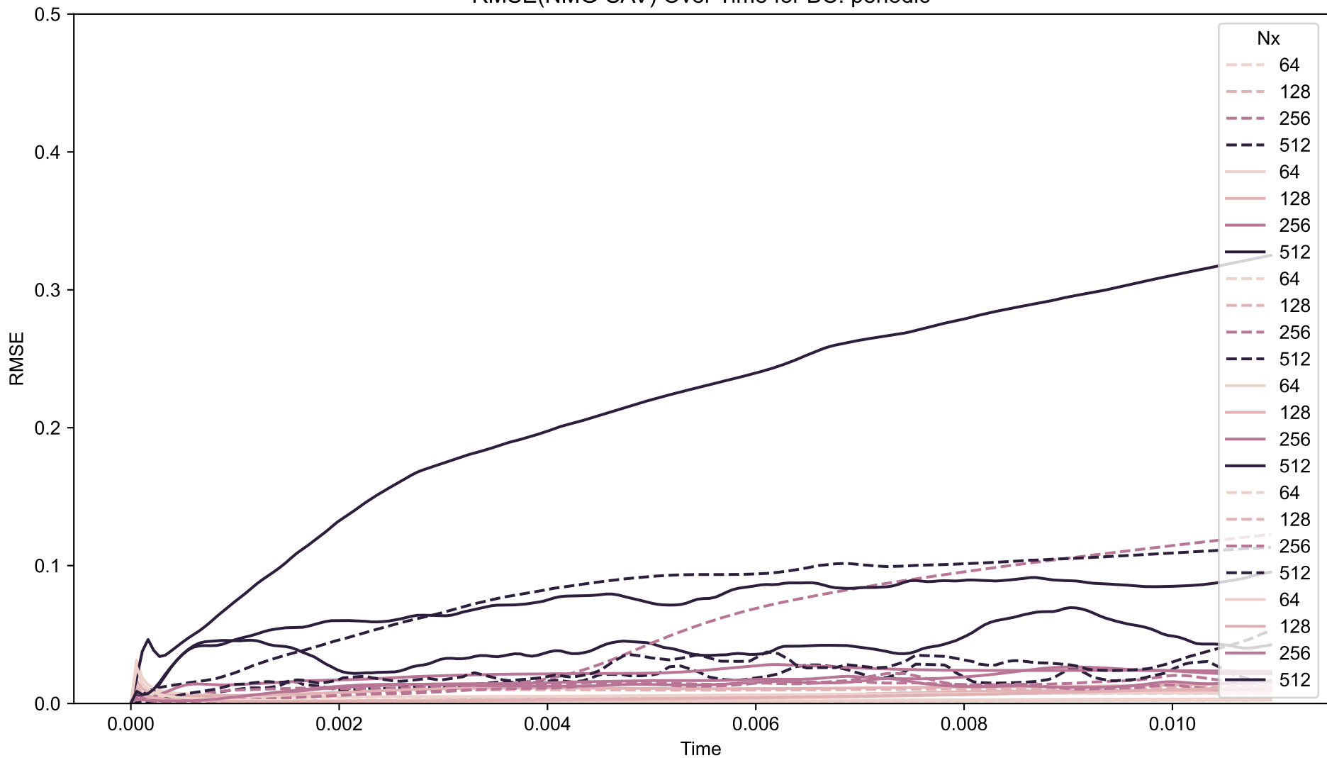
RMSE(NMG-SAV) Over Time for BC: periodic
