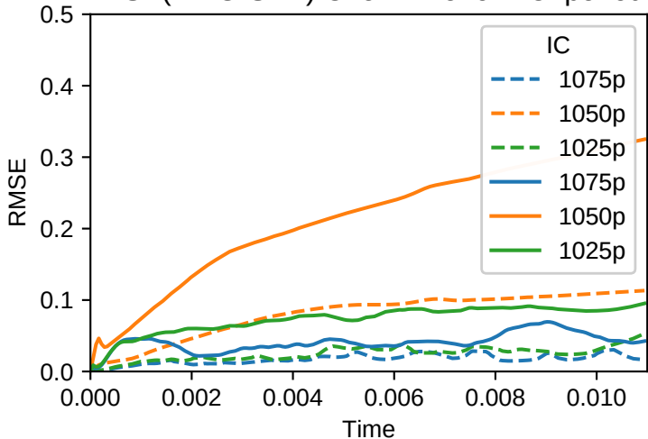
RMSE(NMG-SAV) Over Time for BC: periodic
