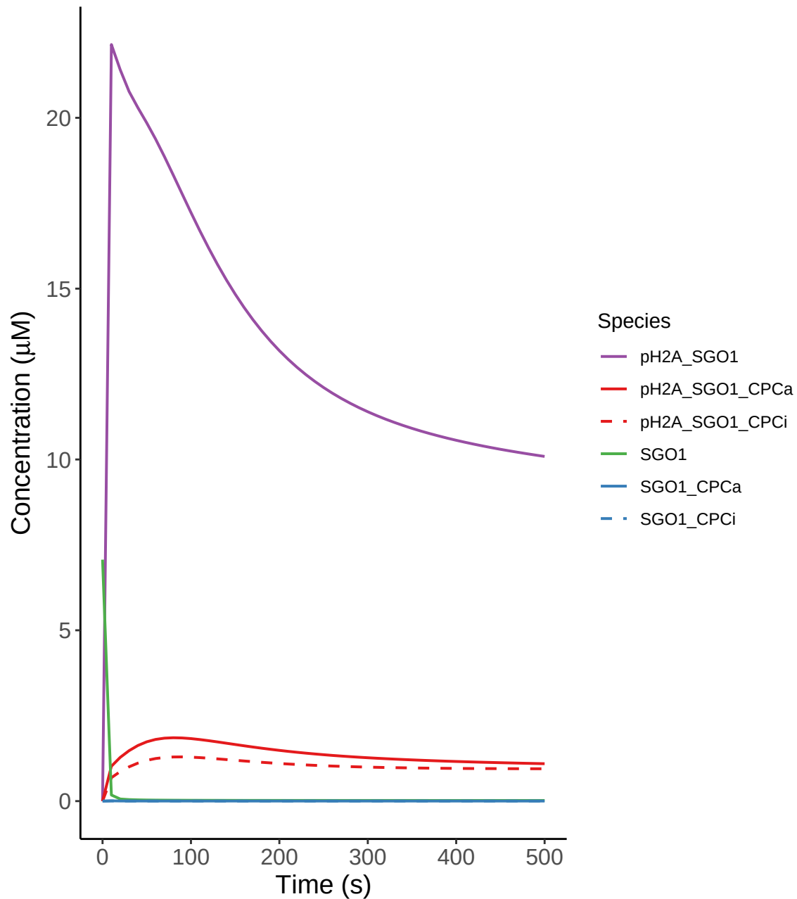
SGO1 Species at inner centromere
