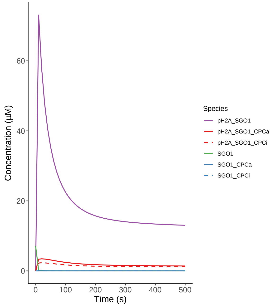
SGO1 Species at kinetochore
