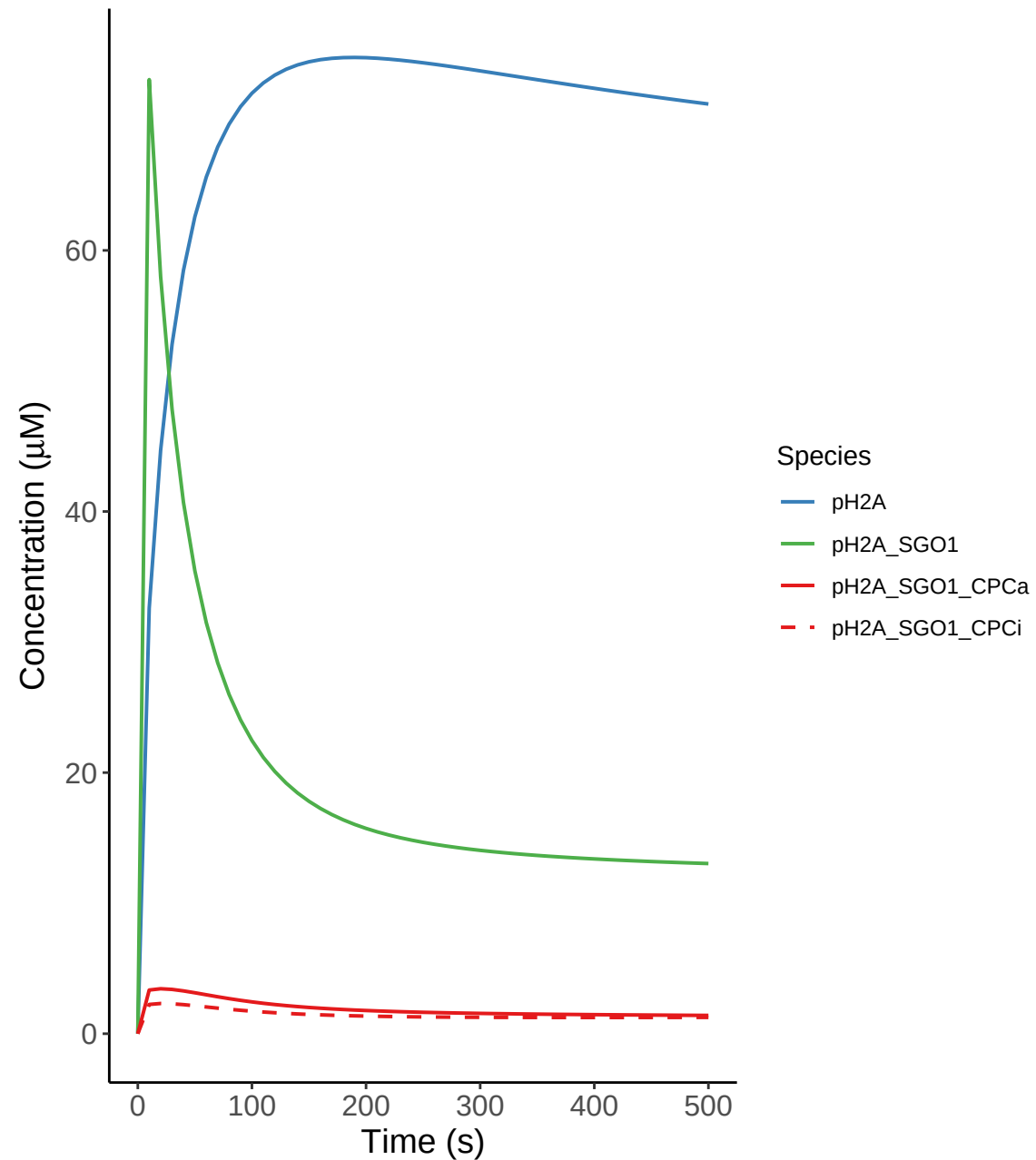
pH2A Species at kinetochore
