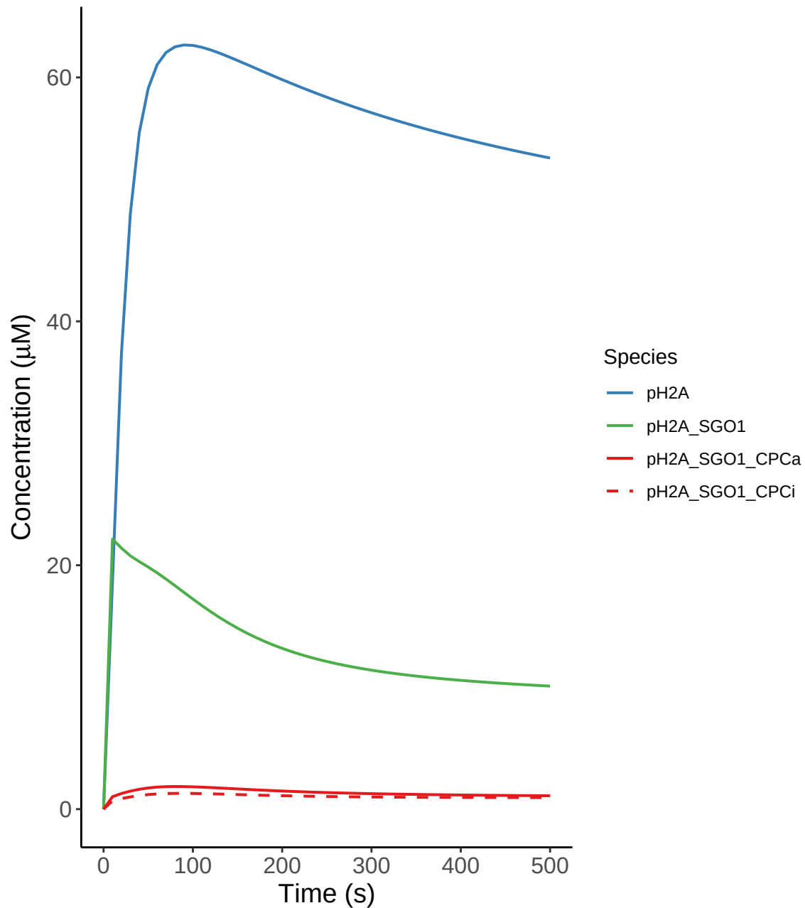
pH2A Species at inner centromere
