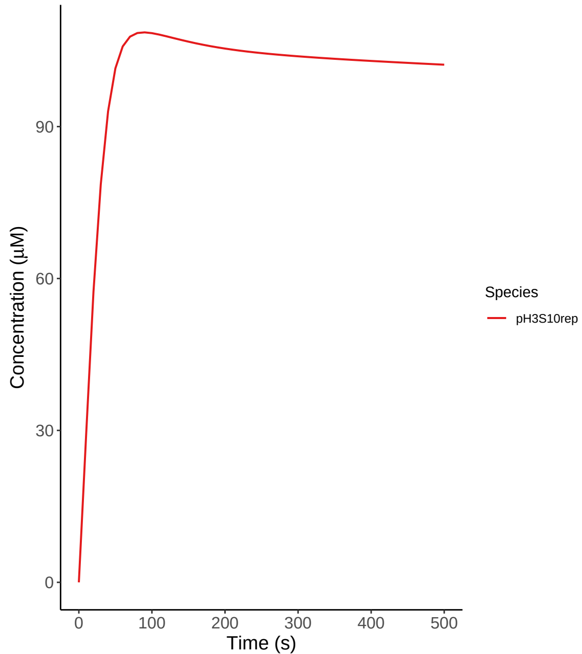
pH3S10 reporter at kinetochore
