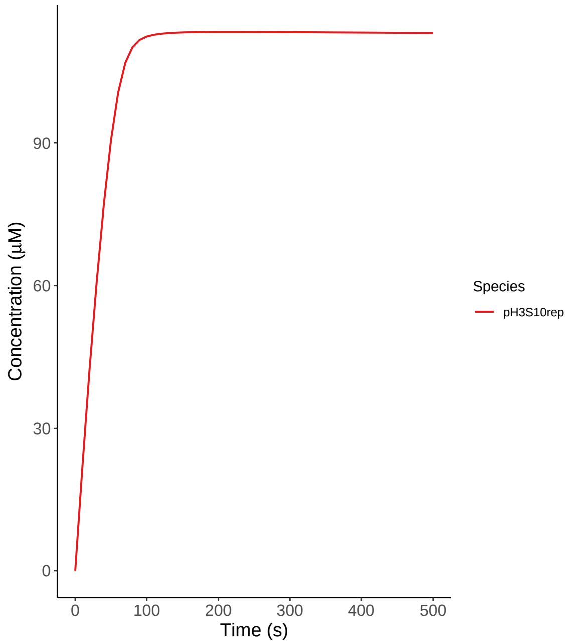
pH3S10 reporter at inner centromere
