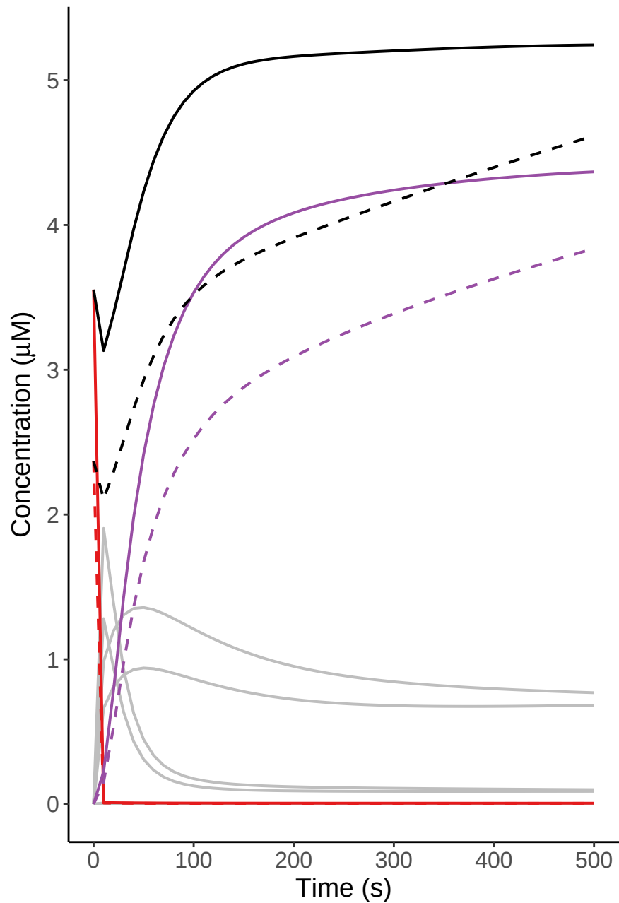
CPC Activation at inner centromere
