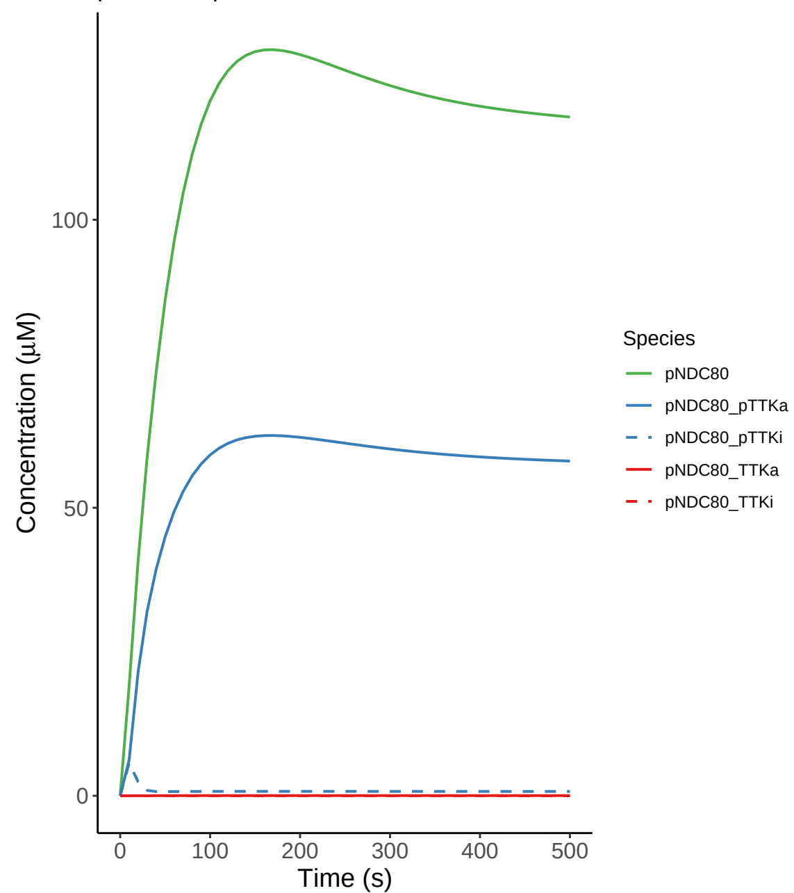
pNDC80 Species at kinetochore
