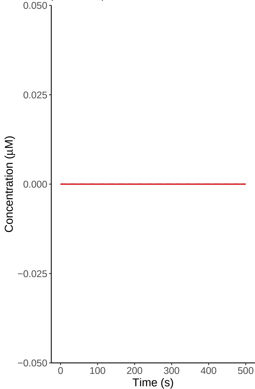
pNDC80 Species at inner centromere
