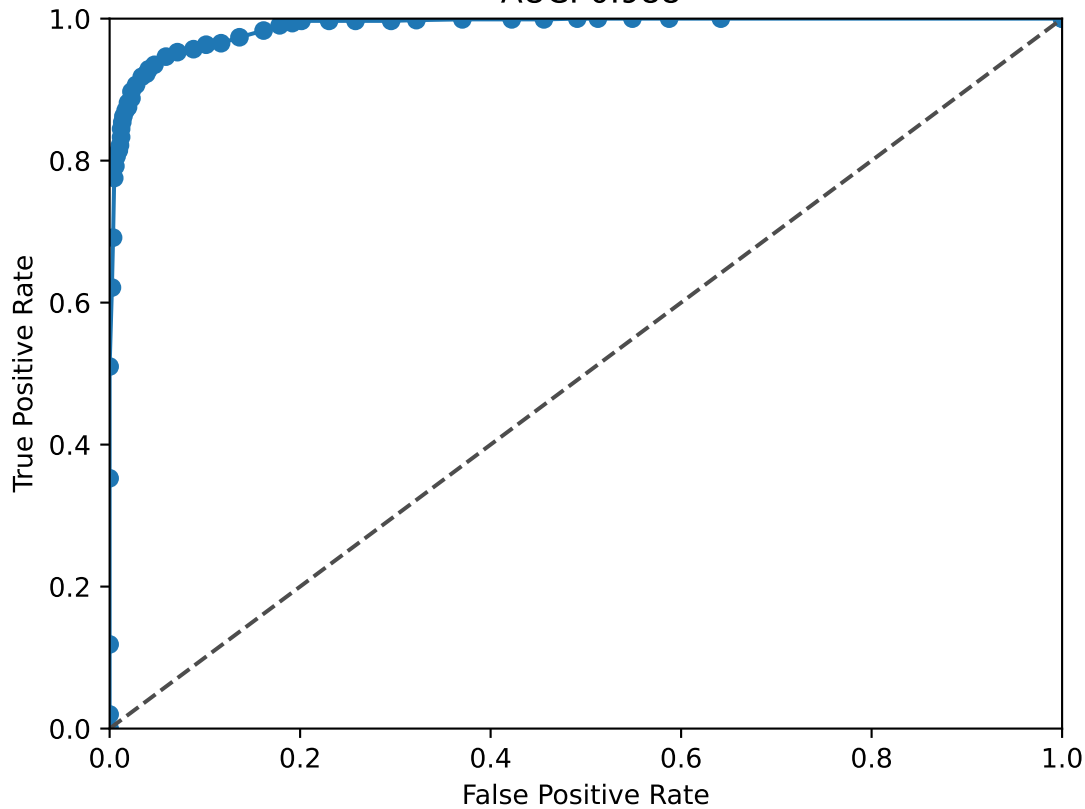
BACH1 ROC Curve AUC: 0.988
