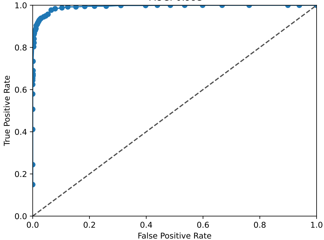
ETS1 ROC Curve AUC: 0.993
