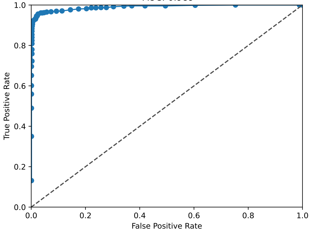
HSF2 ROC Curve AUC: 0.989
