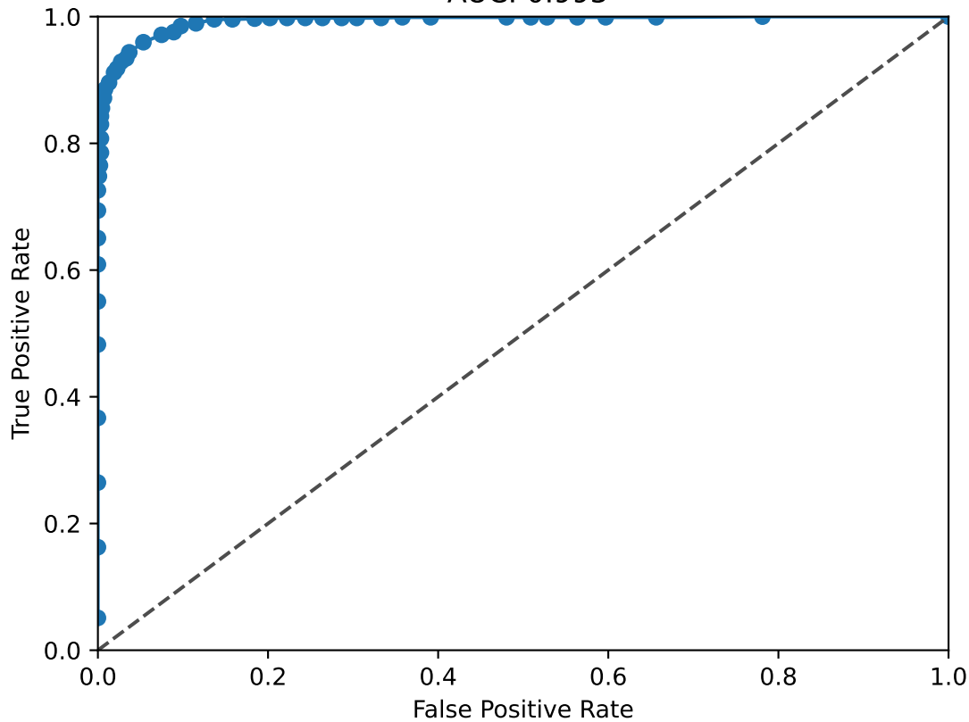
JUN ROC Curve AUC: 0.993
