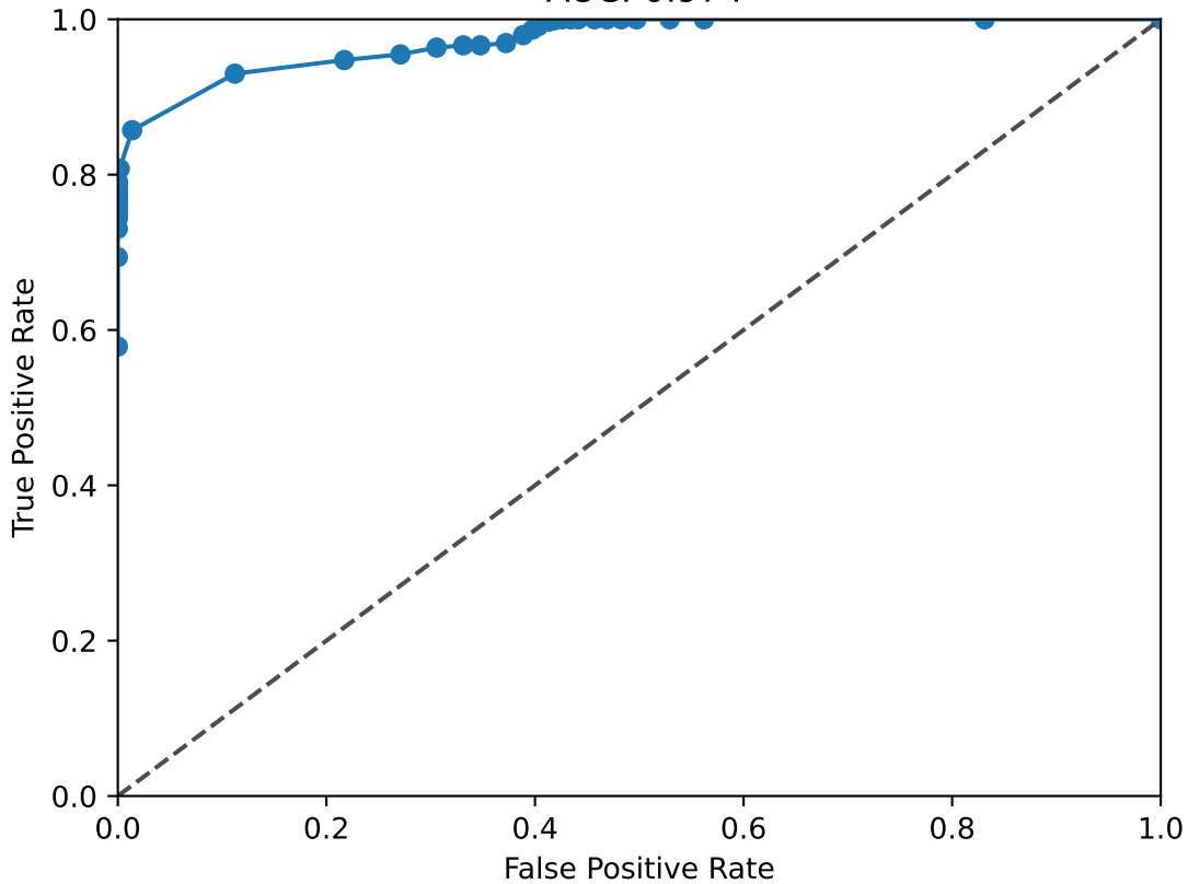
NFIX ROC Curve AUC: 0.974
