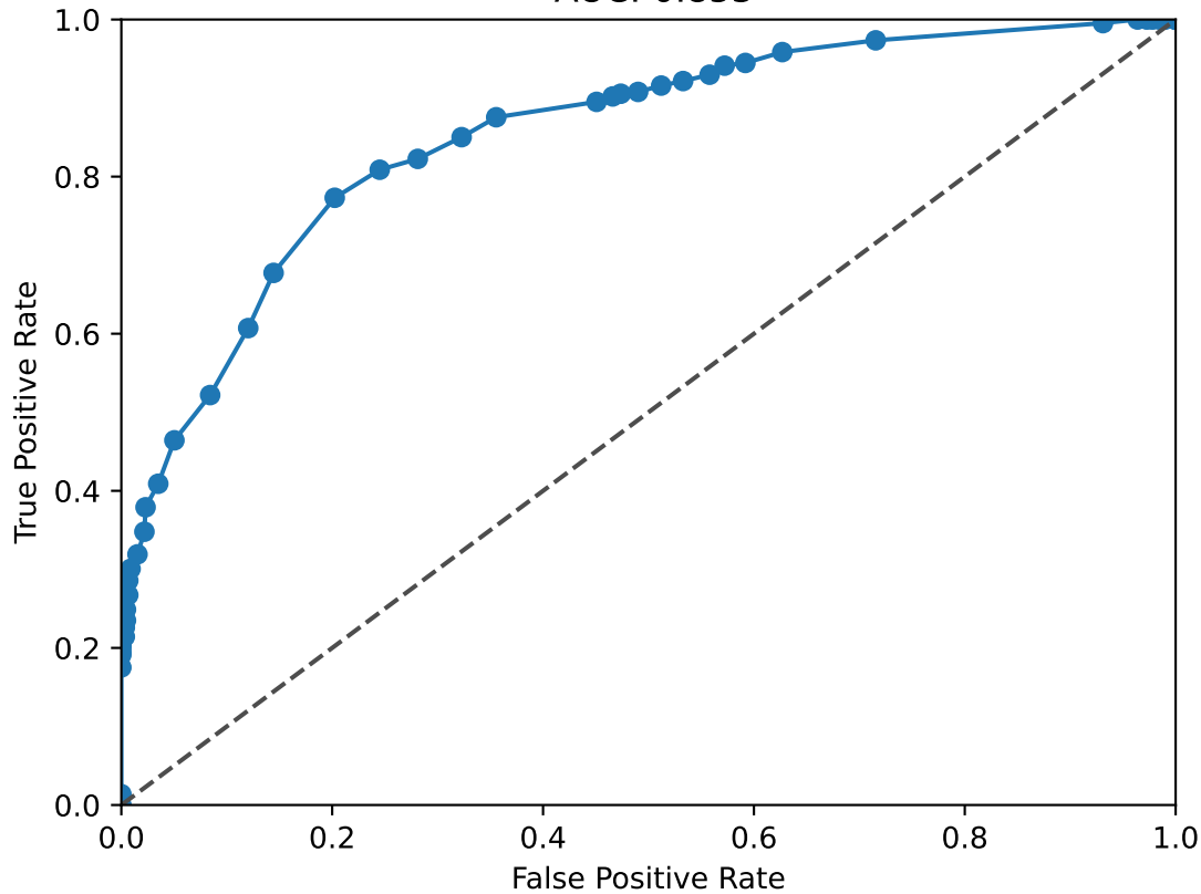
PBX1 ROC Curve AUC: 0.853
