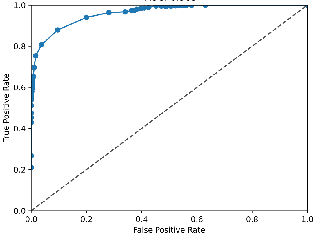
TCF7L1 ROC Curve AUC: 0.963
