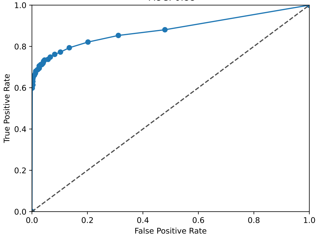
THR B ROC Curve AUC: 0.88
