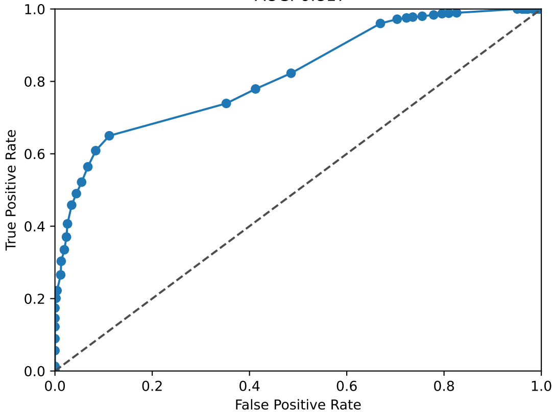
JUNB ROC Curve AUC: 0.817
