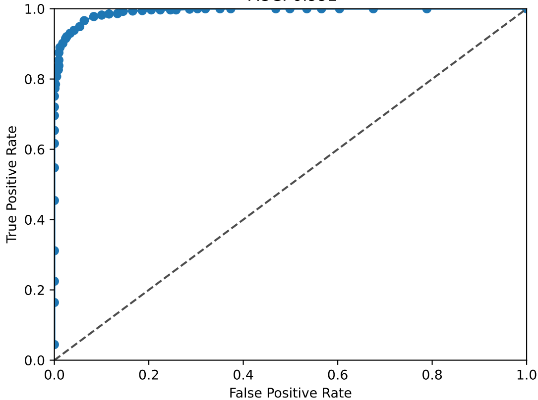
JUN ROC Curve AUC: 0.992
