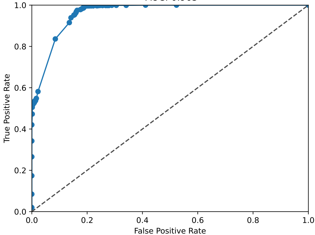
KMT2A ROC Curve AUC: 0.963
