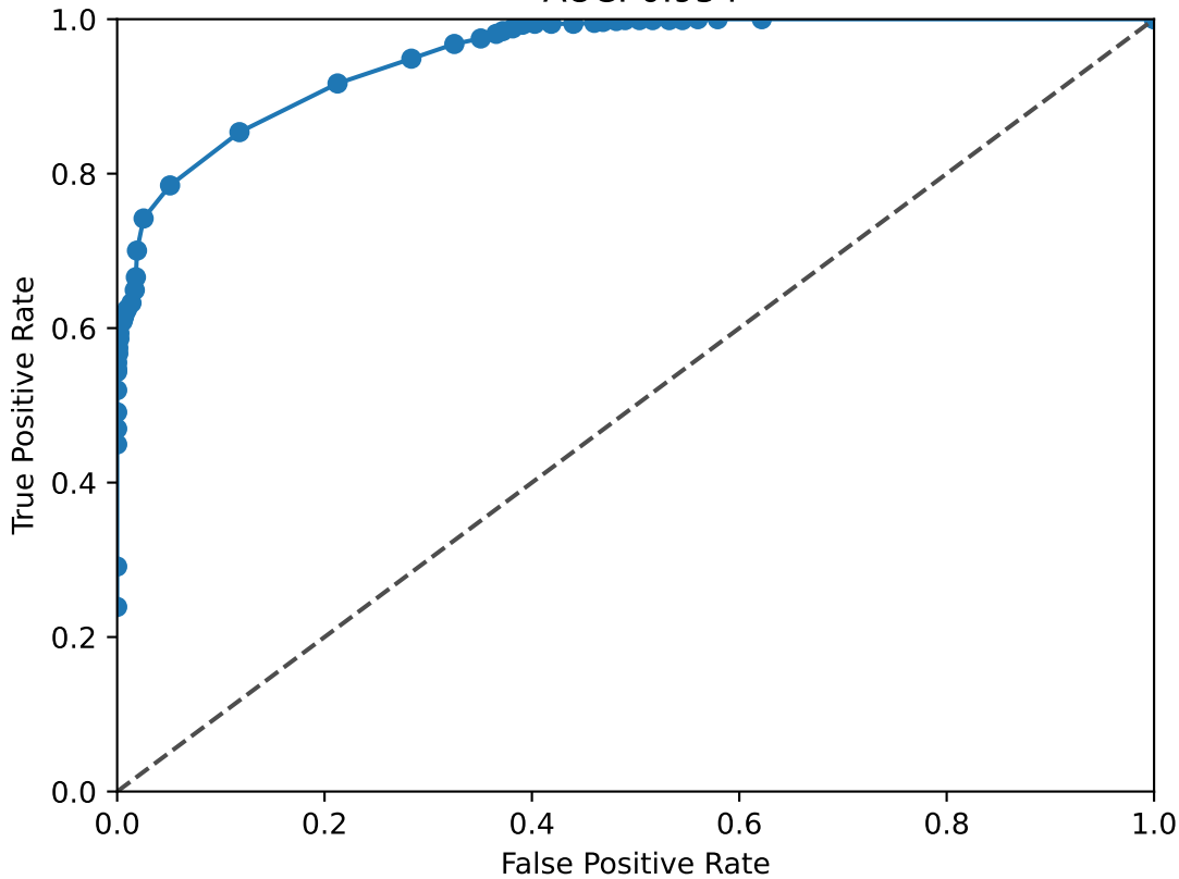
TCF7L1 ROC Curve AUC: 0.954
