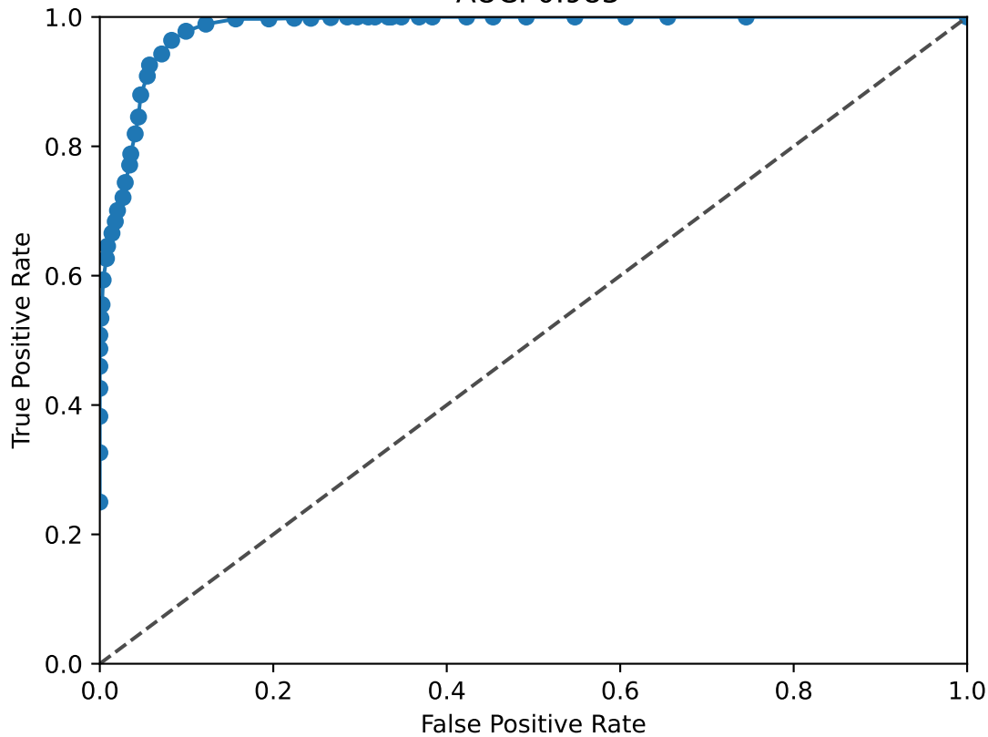
LMX1B ROC Curve AUC: 0.983
