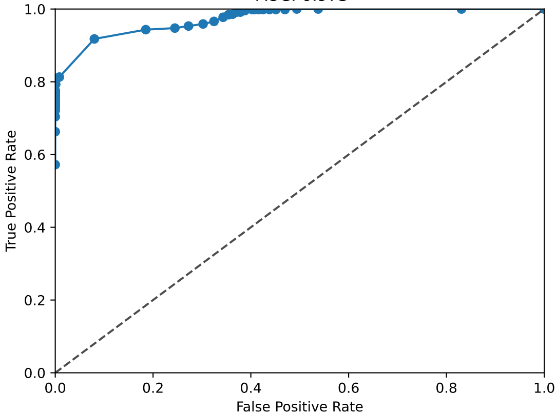
NFIX ROC Curve AUC: 0.973
