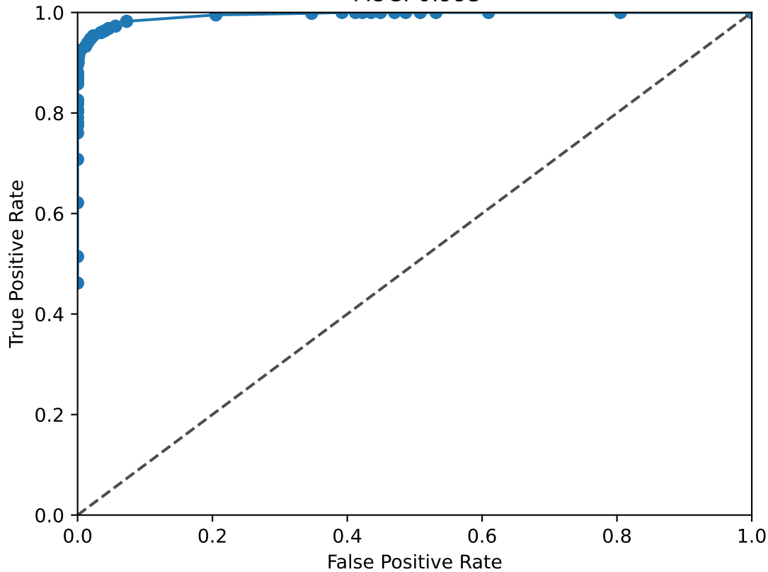
REST ROC Curve AUC: 0.995
