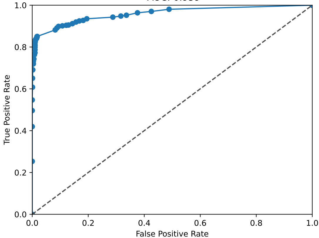
SOX11 ROC Curve AUC: 0.959
