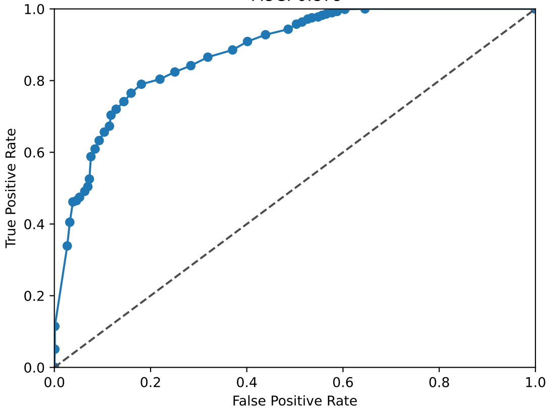
STAT2 ROC Curve AUC: 0.879
