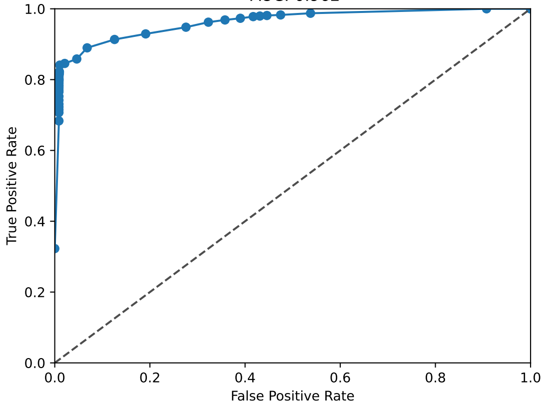
TCF7L2 ROC Curve AUC: 0.962
