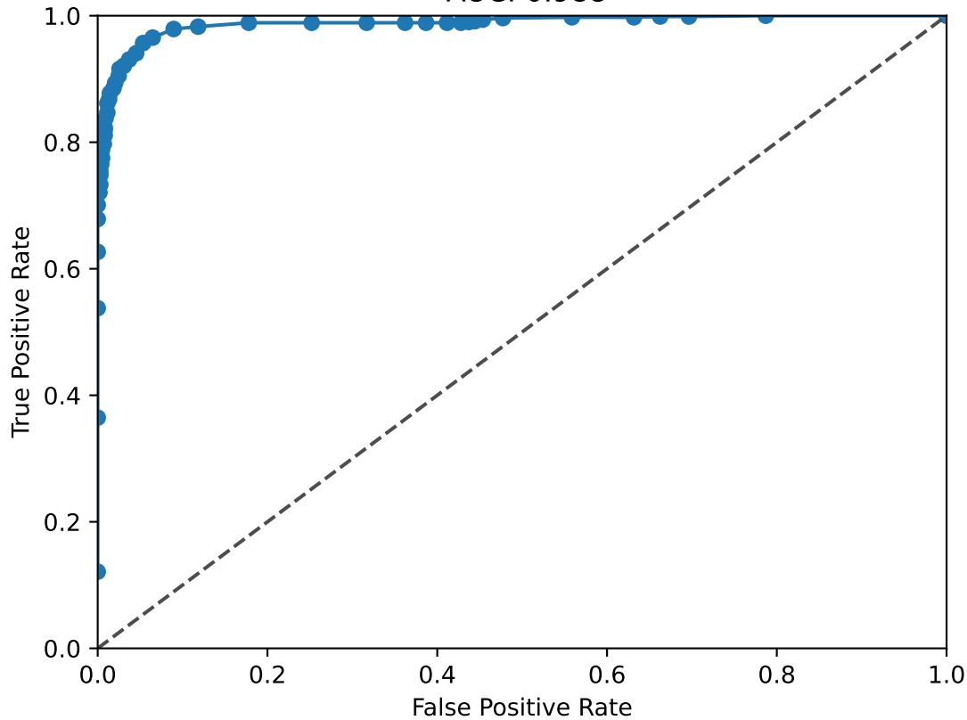
CUX2 ROC Curve AUC: 0.988
