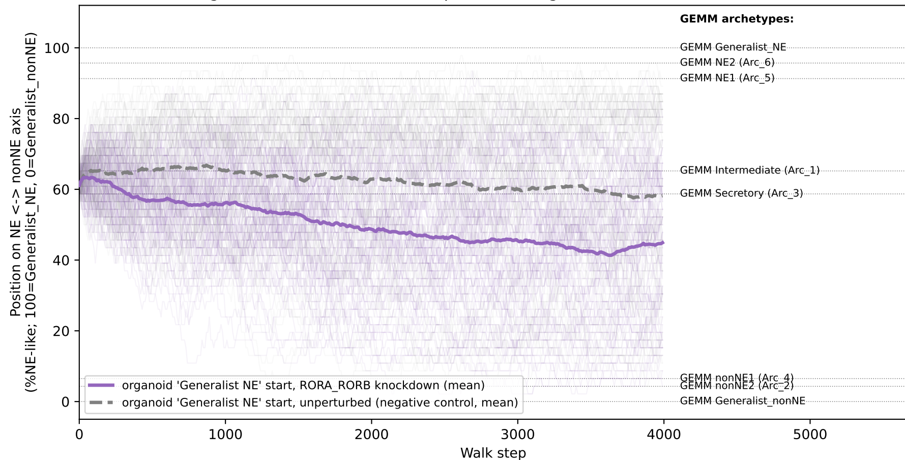
organoid 'Generalist NE' start: position along NE<->nonNE axis over time
