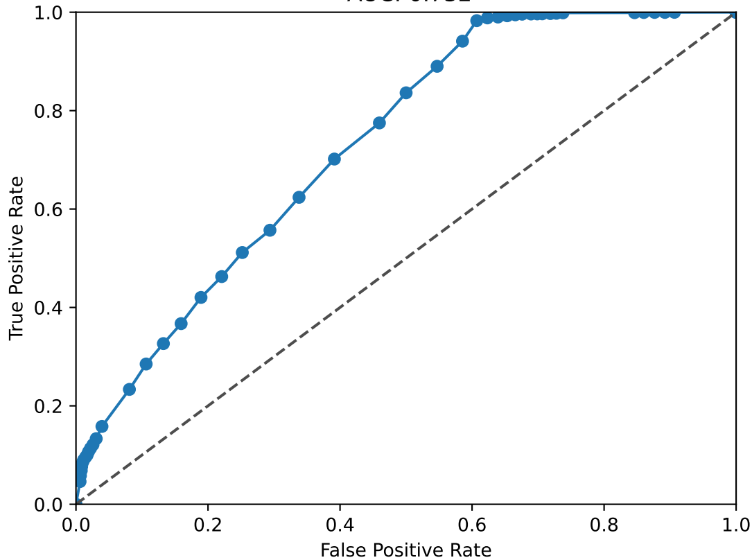
PBX1 ROC Curve AUC: 0.732
