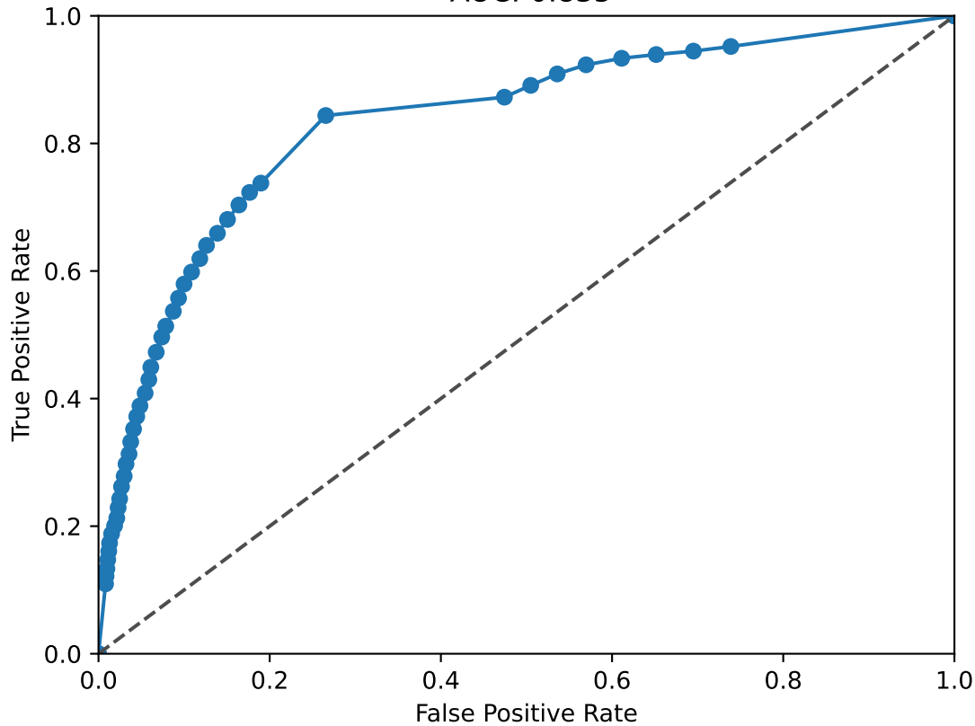
PROX1 ROC Curve AUC: 0.835
