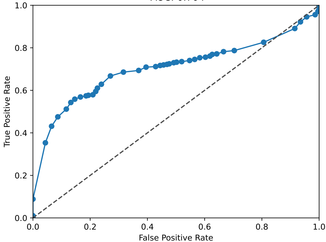
CUX2 ROC Curve AUC: 0.704
