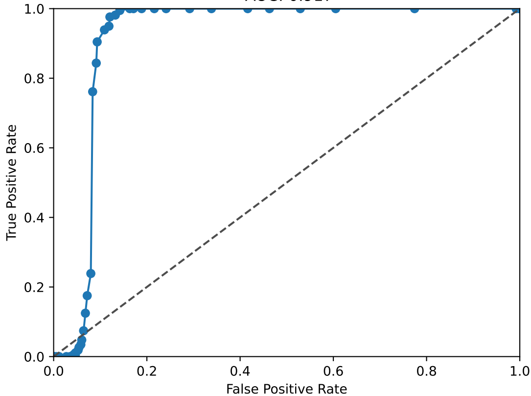
FOXO3 ROC Curve AUC: 0.917
