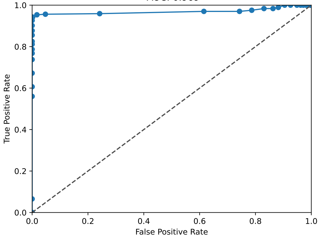
JUN ROC Curve AUC: 0.969
