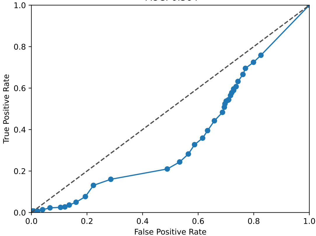
NFIX ROC Curve AUC: 0.364
