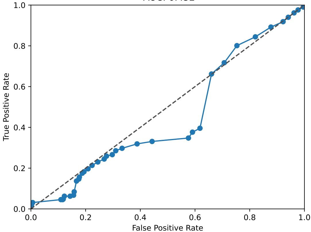
REST ROC Curve AUC: 0.452
