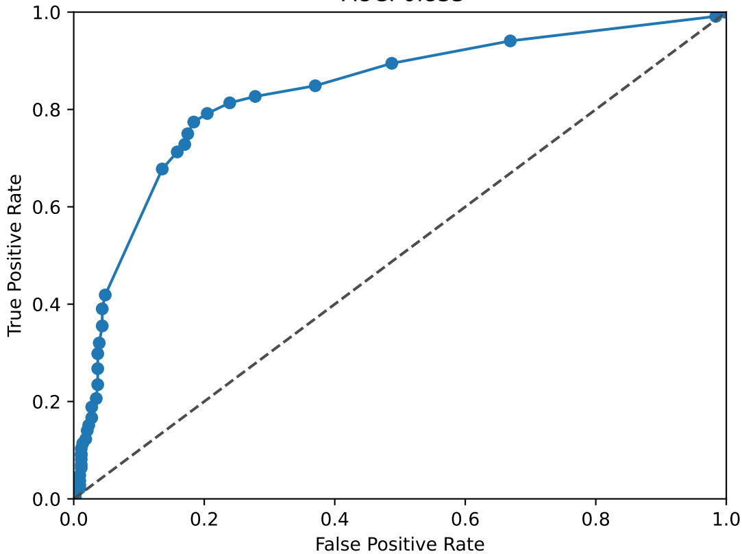
SIX1 ROC Curve AUC: 0.833
