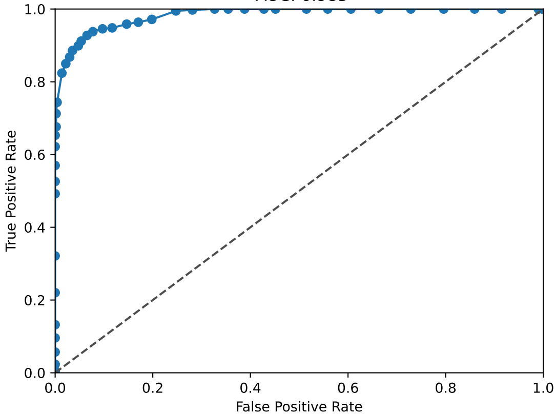
SIX4 ROC Curve AUC: 0.983
