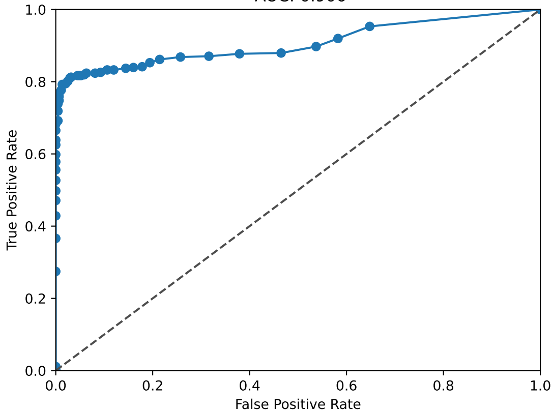
TCF7L1 ROC Curve AUC: 0.906
