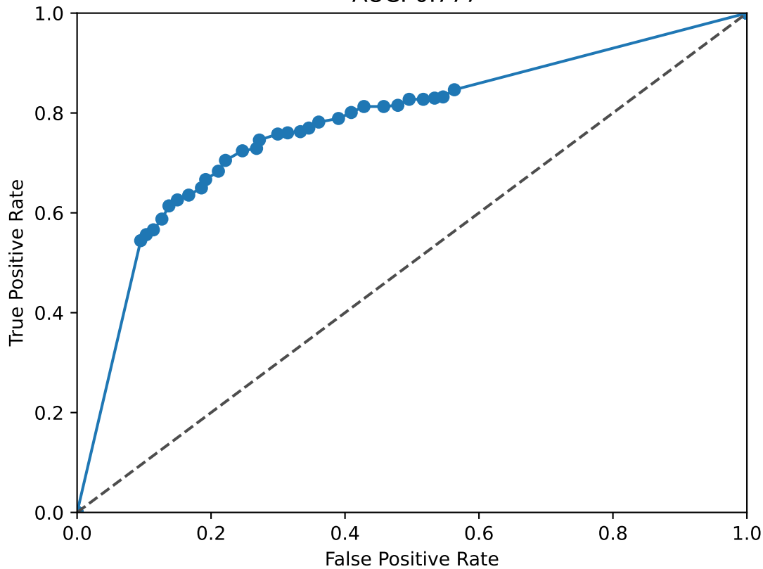
THR B ROC Curve AUC: 0.777
