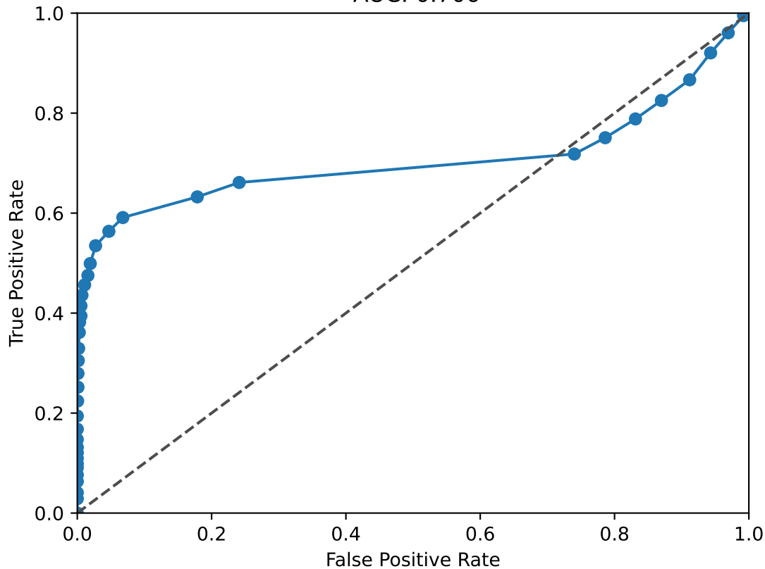
BACH2 ROC Curve AUC: 0.706
