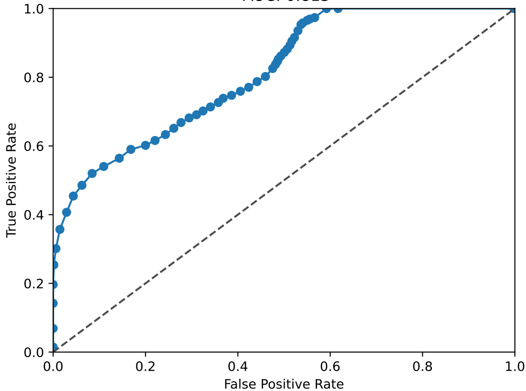
HSF2 ROC Curve AUC: 0.813
