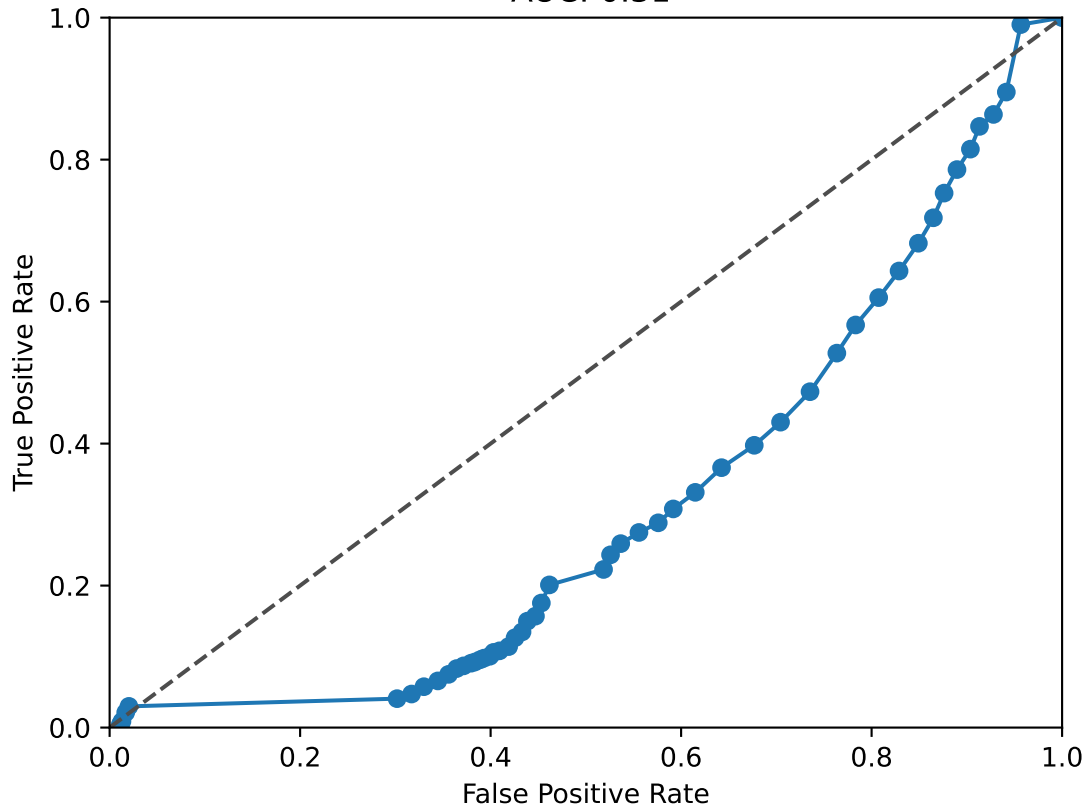
NFIX ROC Curve AUC: 0.31
