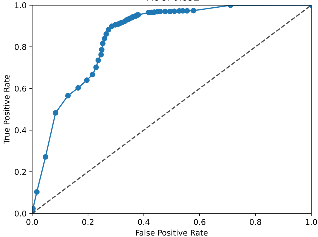
NFKB1 ROC Curve AUC: 0.852
