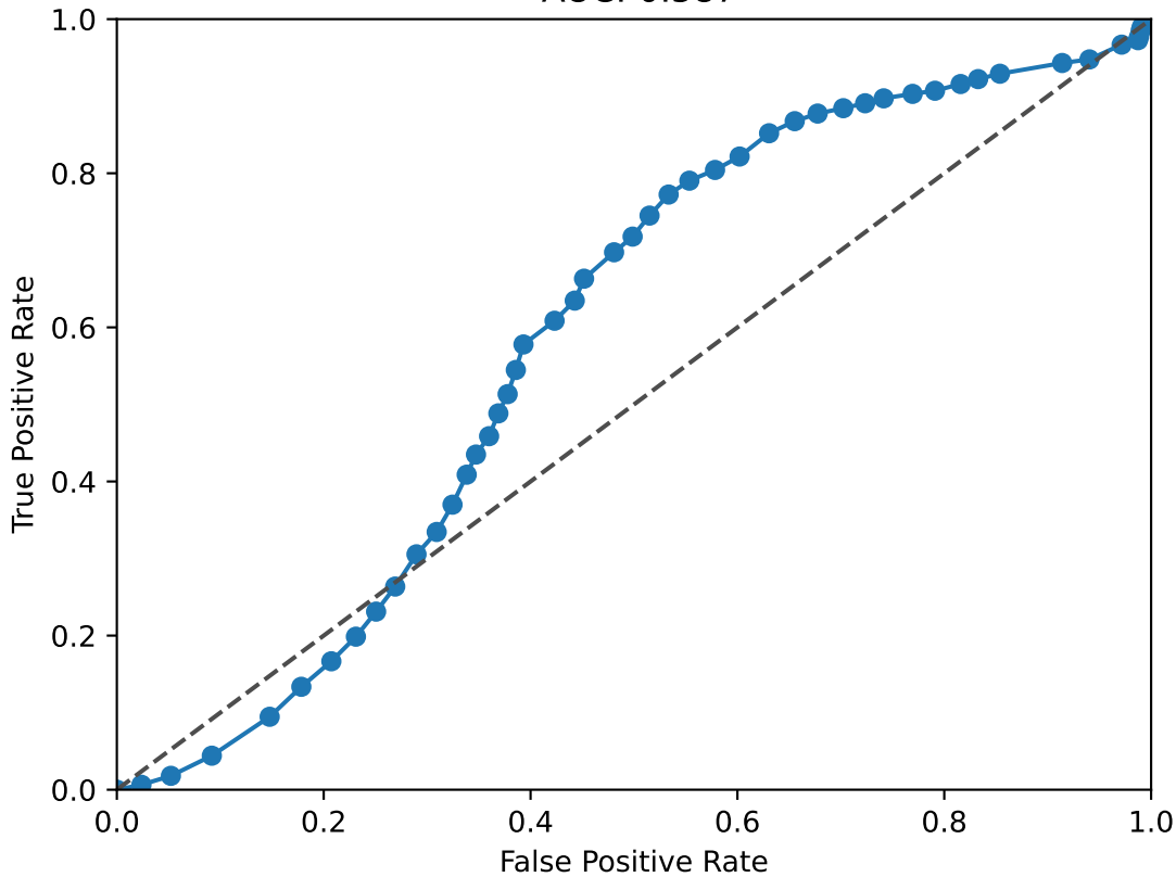
PKNOX2 ROC Curve AUC: 0.587
