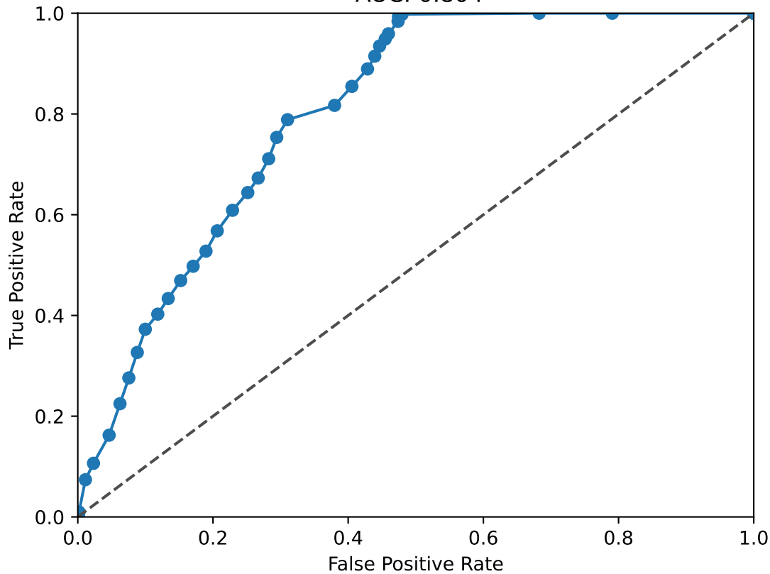
SOX11 ROC Curve AUC: 0.804
