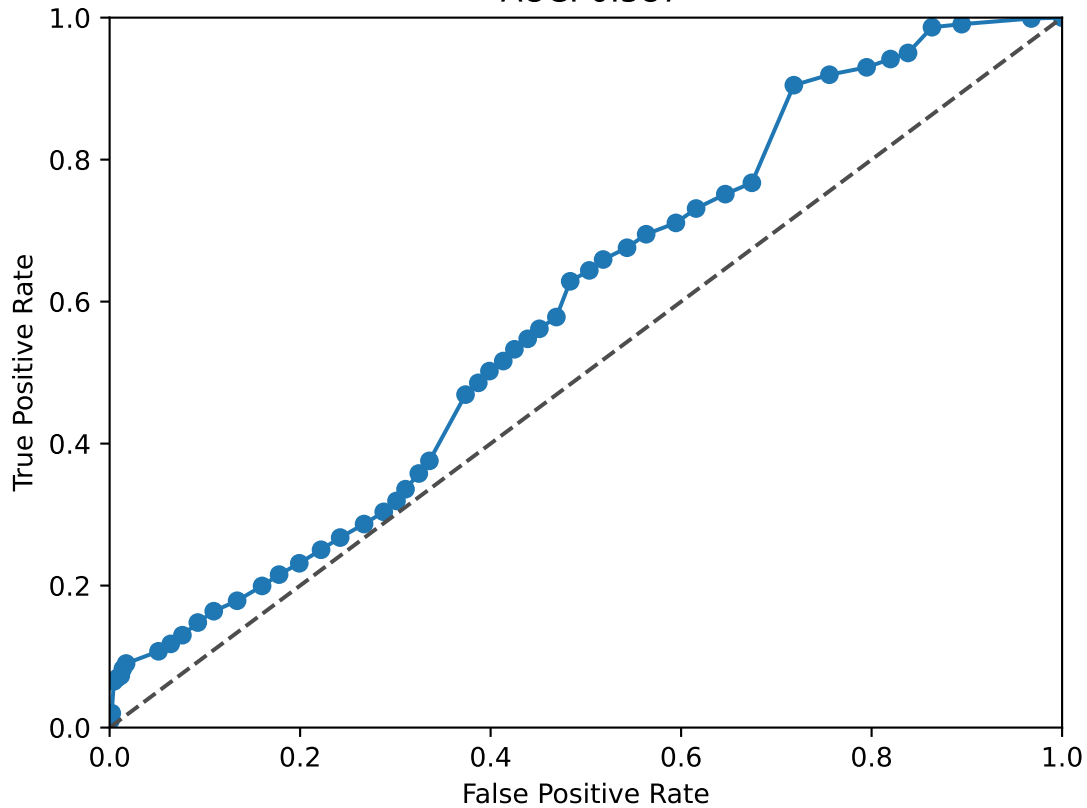
ETS1 ROC Curve AUC: 0.587
