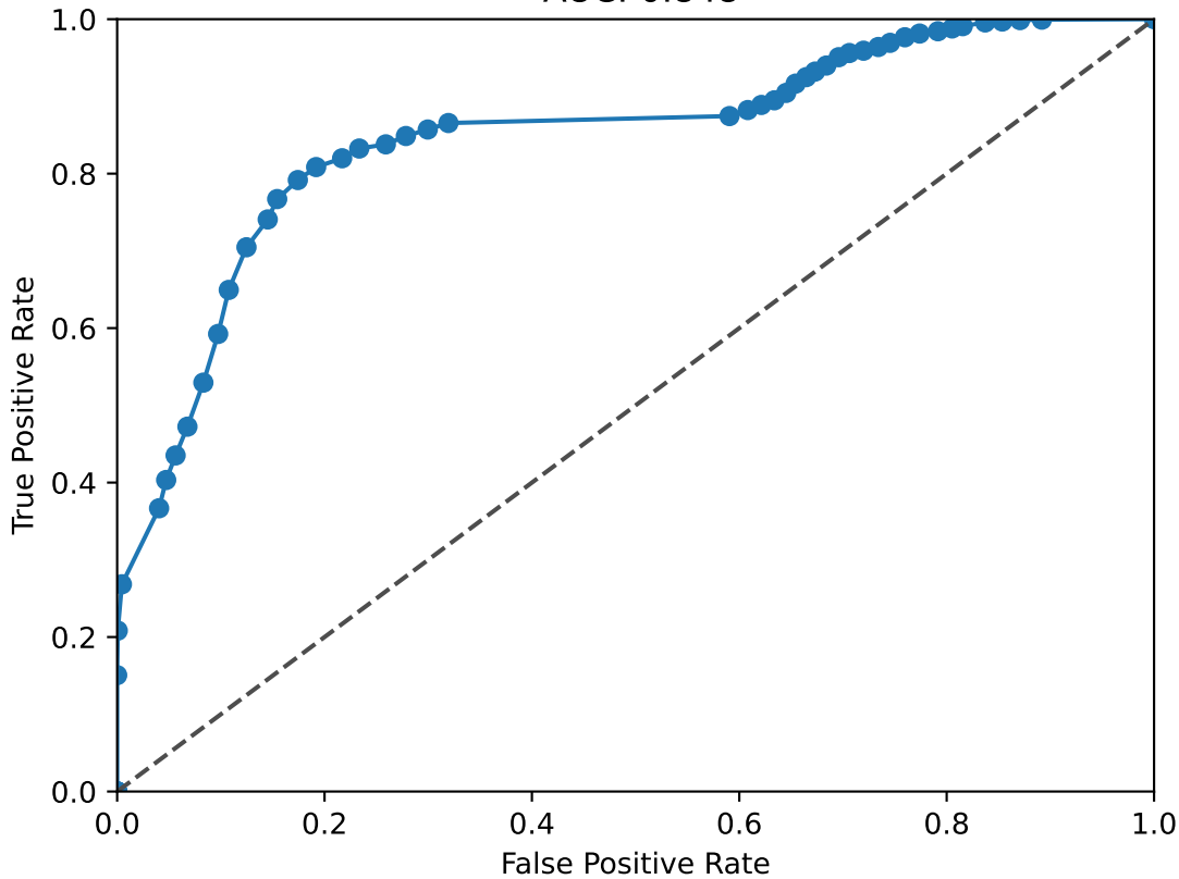
JUNB ROC Curve AUC: 0.848
