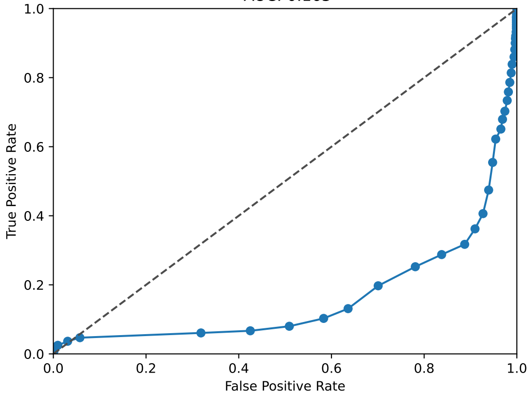
KMT2A ROC Curve AUC: 0.163
